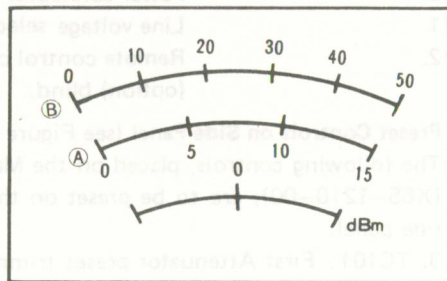
Figure 5 – Meter Scale Graduations.
